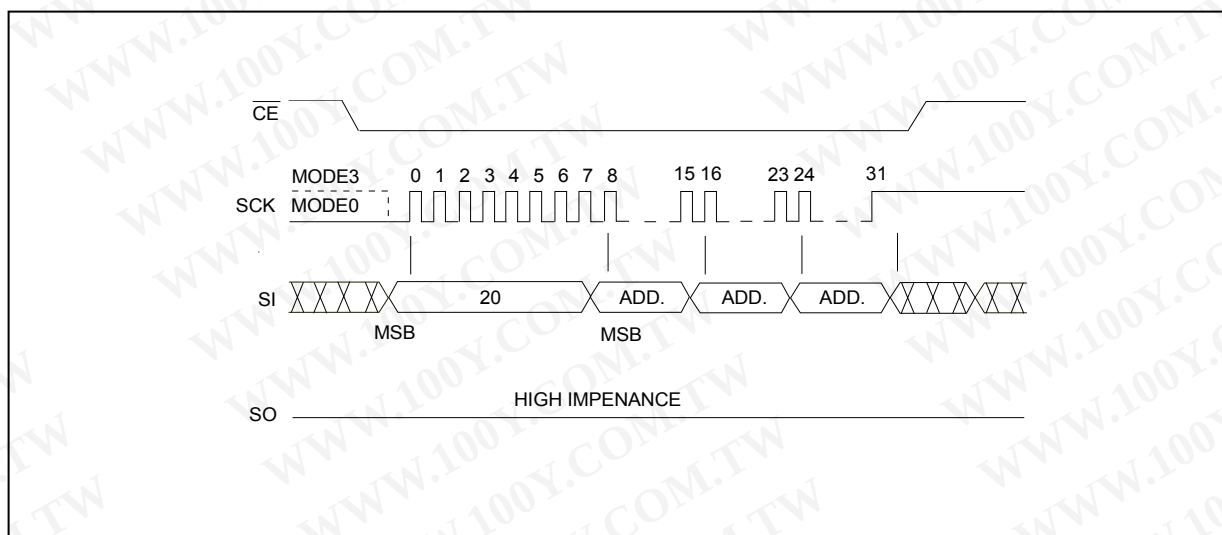
FIGURE 10 : SEQUENCE-ERASE SEQUENCE
