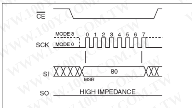
FIGURE 6 : DISABLE SO AS HARDWARE RY/RY DURING AAI PROGRAMMING
