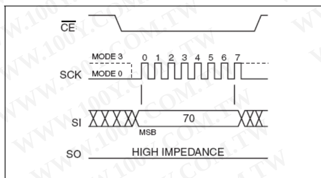
FIGURE 5 : ENABLE SO AS HARDWARE RY/RY DURING AAI PROGRAMMING
