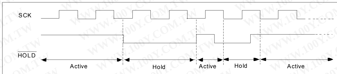
Figure 1 : HOLD CONDITION WAVEFORM
