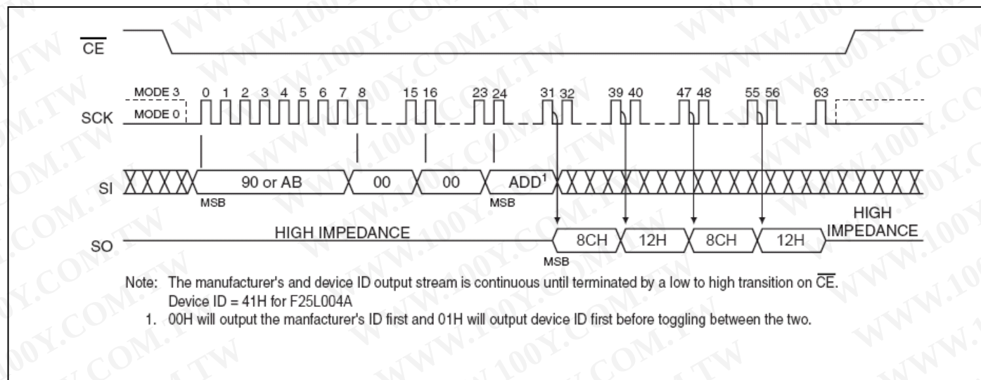
Figure 18 : Read-Electronic-Signature
