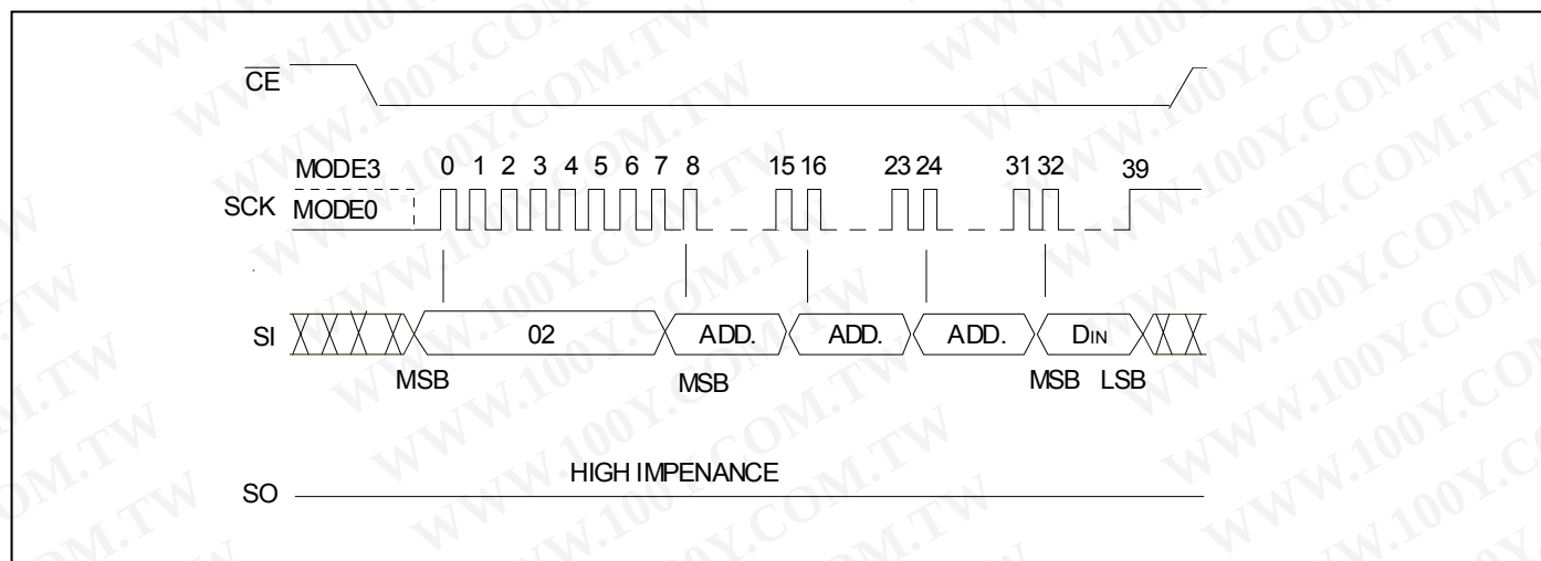
Figure 4 : BYTE-PROGRAM SEQUENCE
