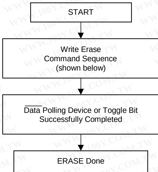
Flowchart 3. Embedded Erase
