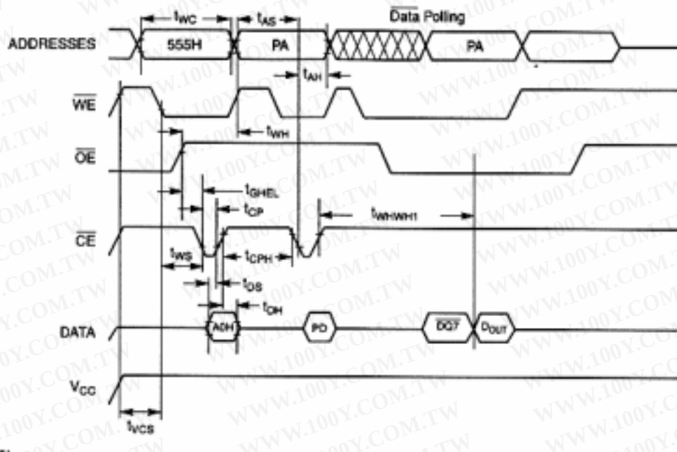
Figure 10. Alternate /CE Controlled Write Operation Timings
