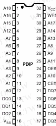
FIGURE 2. PDIP
