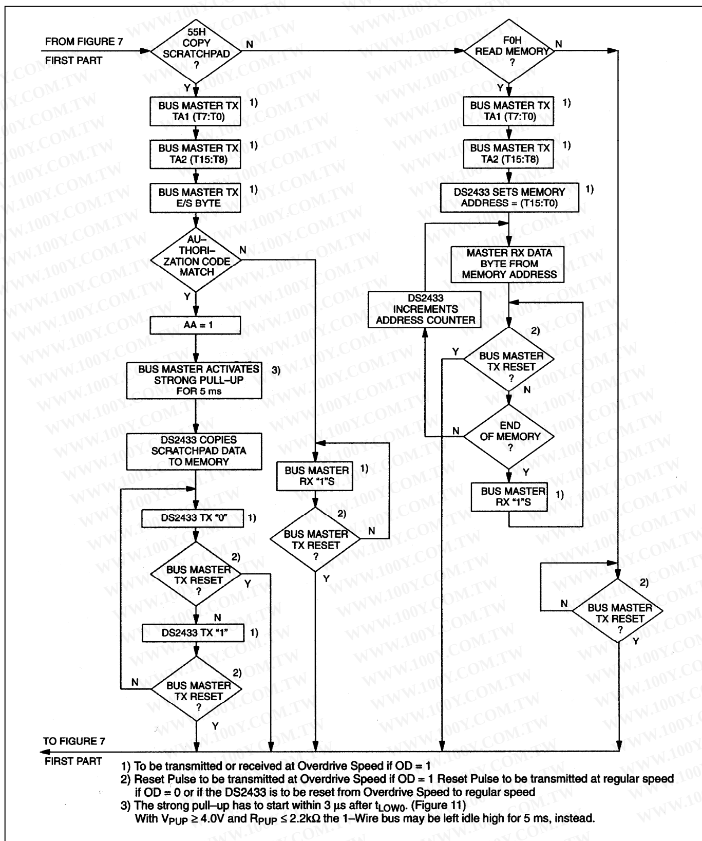
Figure 7. MEMORY FUNCTION FLOWCHART (continued)
