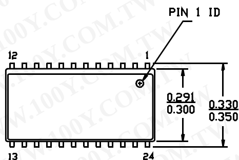
24-Lead (300-Mil) Molded SOJ V1
