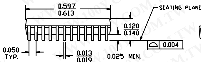
28-Lead (300-Mil) Molded SOJ V21
