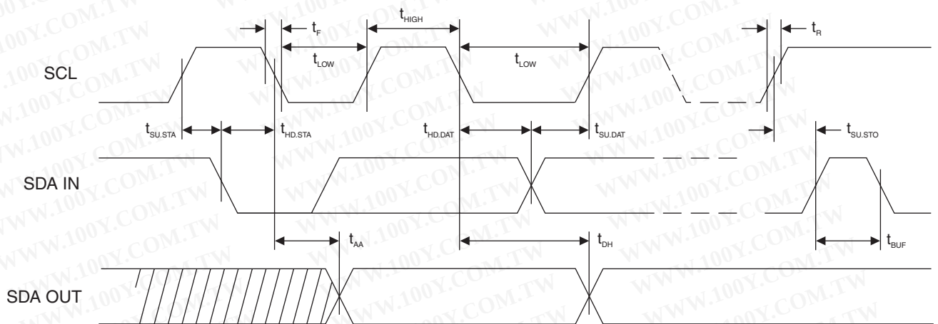
Figure 6-4. Bus Timing
