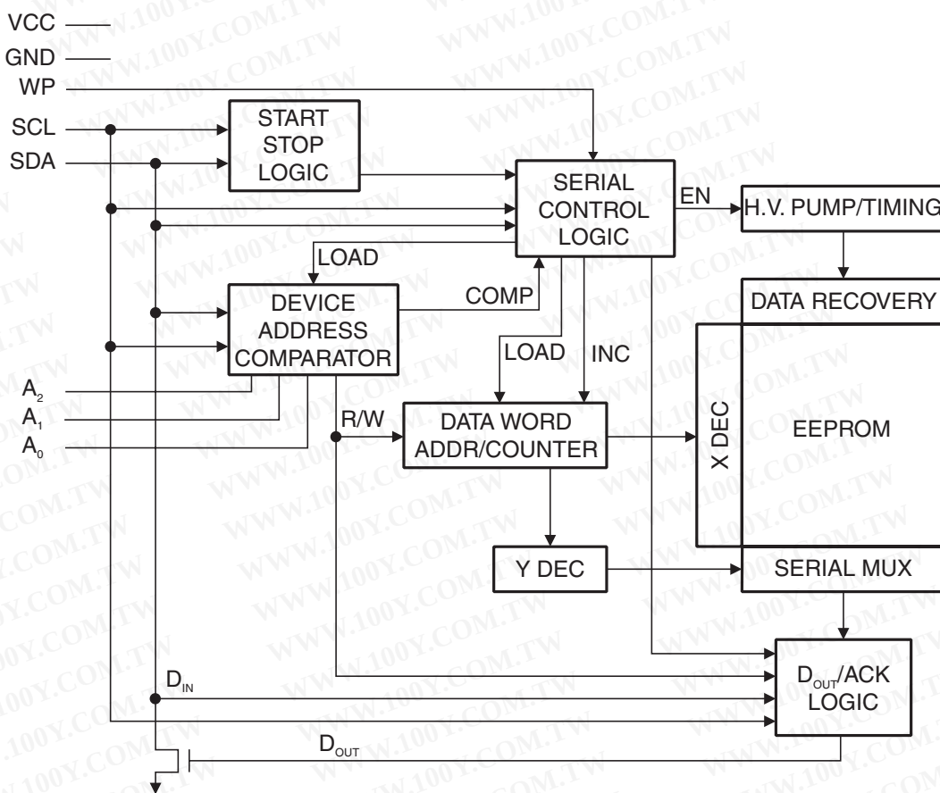
Figure 3-1. Block Diagram
