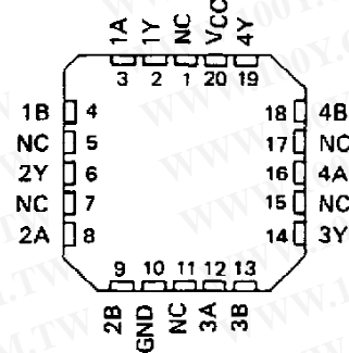
SN54LS02, SN54S02 . . . FK PACKAGE (TOP VIEW)
