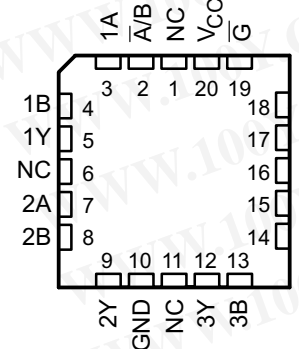
SN54AHC157 ... FK PACKAGE (TOP VIEW)
