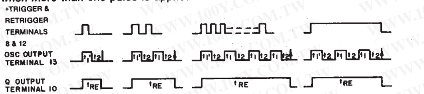
Fig. 34—Retrigger-mode waveforms.
