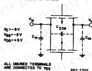
Fig. 24 - Capacitance C_{IOS} and C_{OS} .
