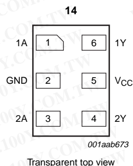
Fig.2 Pin configuration XSON6.
