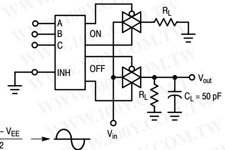
Figure 8. Channel Separation (Adjacent Channels Used For Setup)
