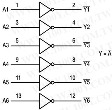
Figure 1. Logic Diagram
