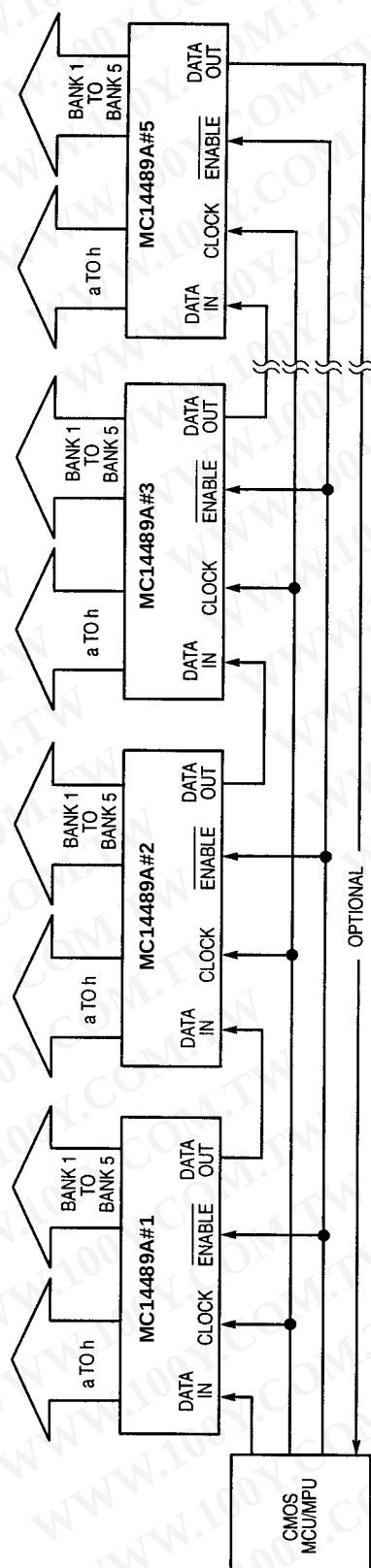
(a) Cascading Five Devices
