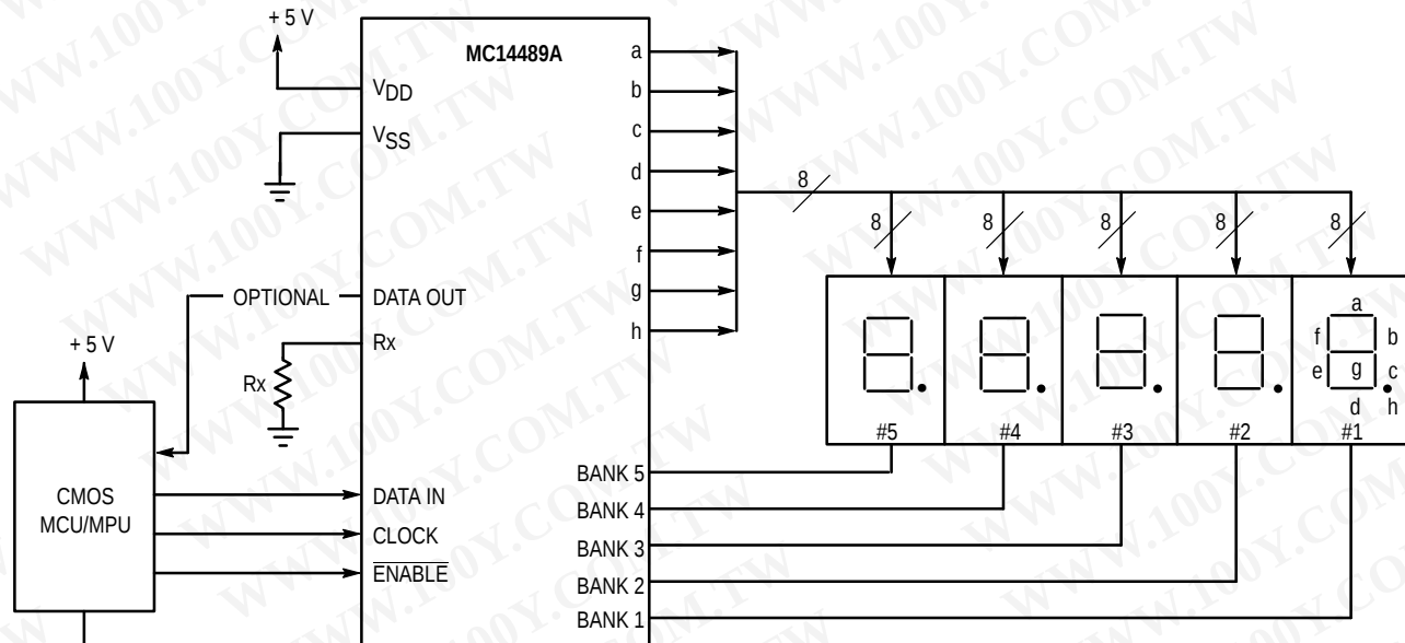
Figure 9. Non-Cascaded Application Example: 5 Character Common Cathode LED Display with Two Intensities as Controlled via Serial Port
