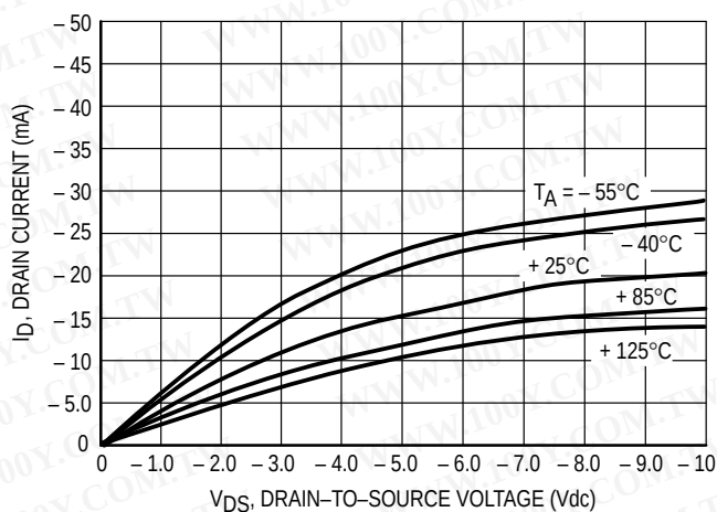
Figure 5. V_{GS} = -10 Vdc
