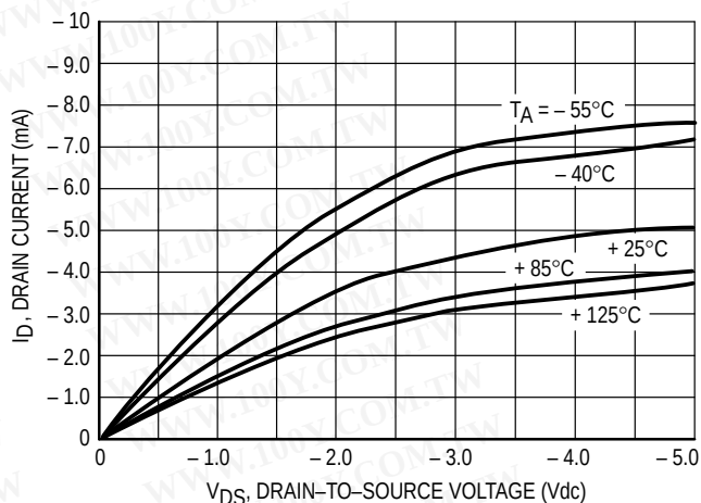
Figure 3. V_{GS} = -5.0 Vdc
