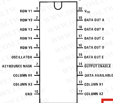
Top View MM74C923
