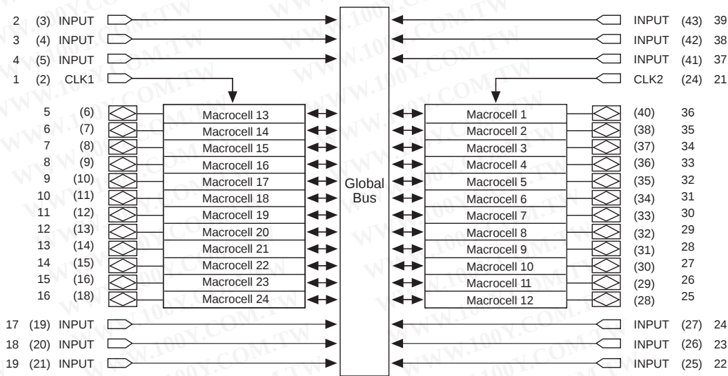
Figure 12. EP910 Block Diagram
