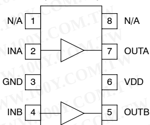
D, DGN, OR P PACKAGE (TOP VIEW)
