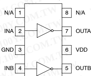
D, DGN, OR P PACKAGE (TOP VIEW)
