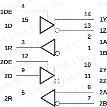
SN65C1168, SN75C1168
