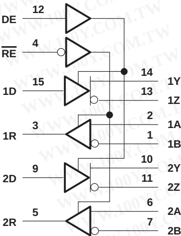
SN65C1167/SN75C1167
