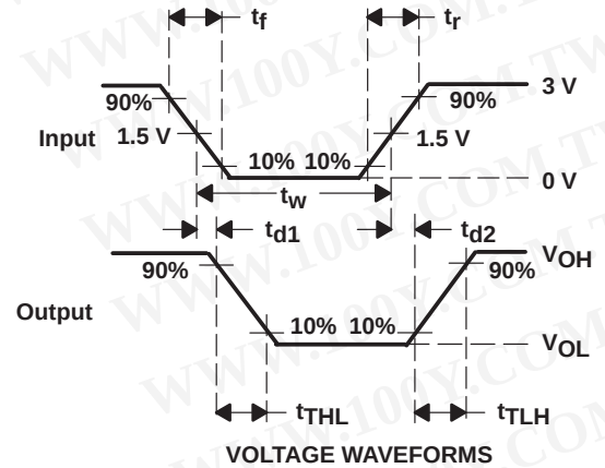
Figure 1. Test Circuit and Switching Times From Data Inputs
