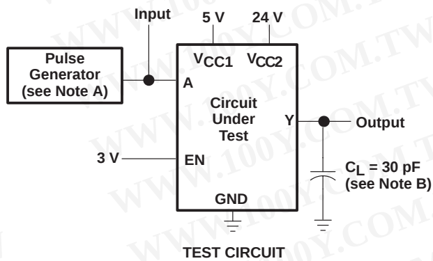
Figure 1. Test Circuit and Switching Times From Data Inputs
