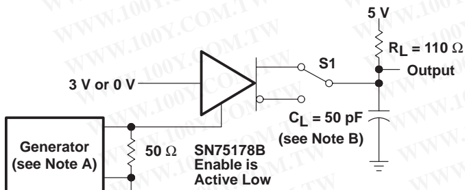
TEST CIRCUIT
