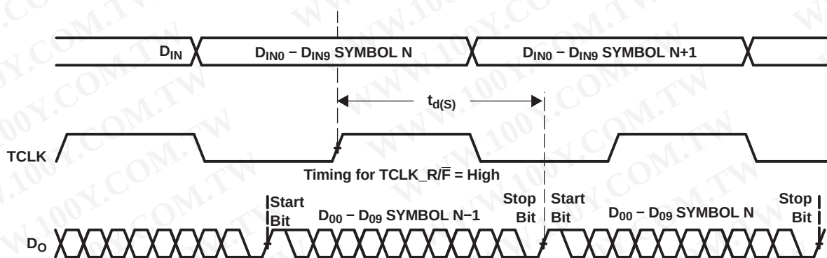
Figure 13. Serializer Delay
