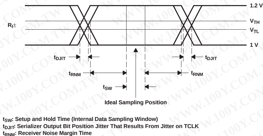
Figure 19. Receiver LVDS Input Skew Margin
