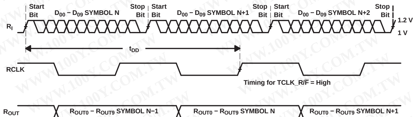
Figure 14. Deserializer Delay
