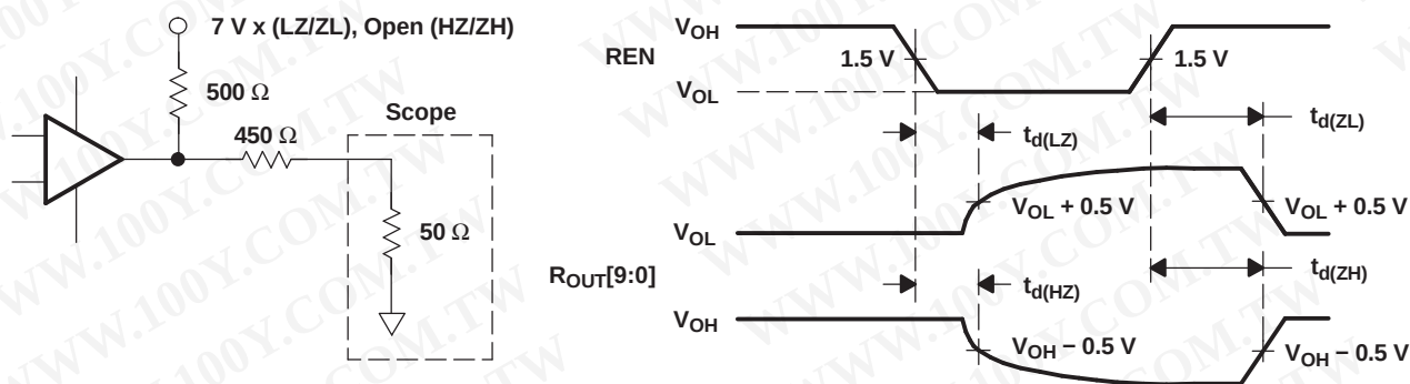
Figure 16. Deserializer High-Impedance State Test Circuit and Timing
