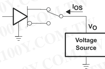
Figure 9. Driver Short-Circuit Test
