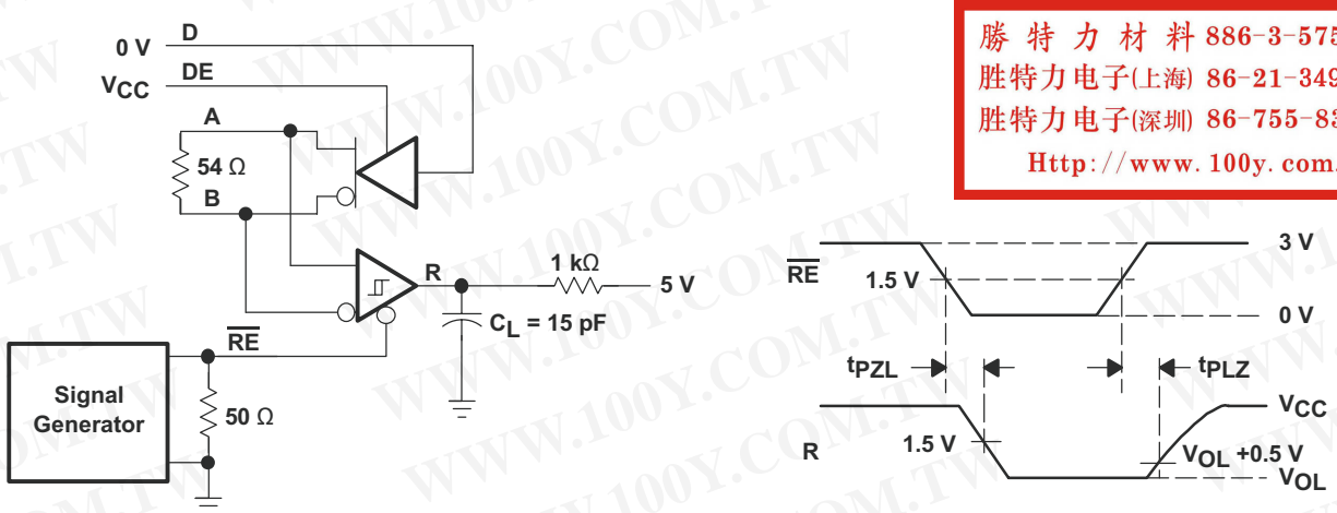
Figure 13. Receiver Enable Test Circuit and Waveforms, Data Output Low
