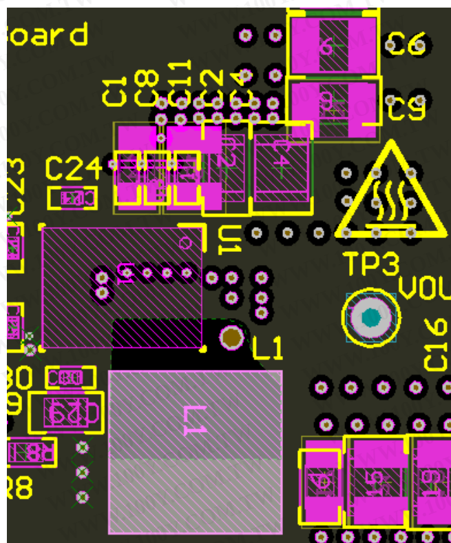
Figure 17. Ground Plane
