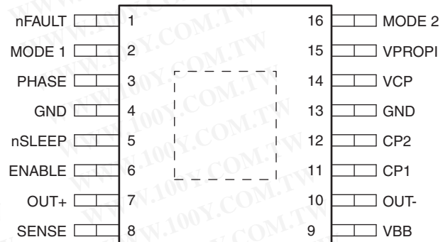
DRV8801 PWP PACKAGE (TOP VIEW)
