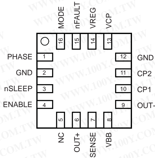
DRV8800 RTY PACKAGE (TOP VIEW)
