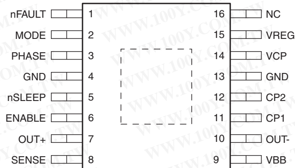
DRV8800 PWP PACKAGE (TOP VIEW)
