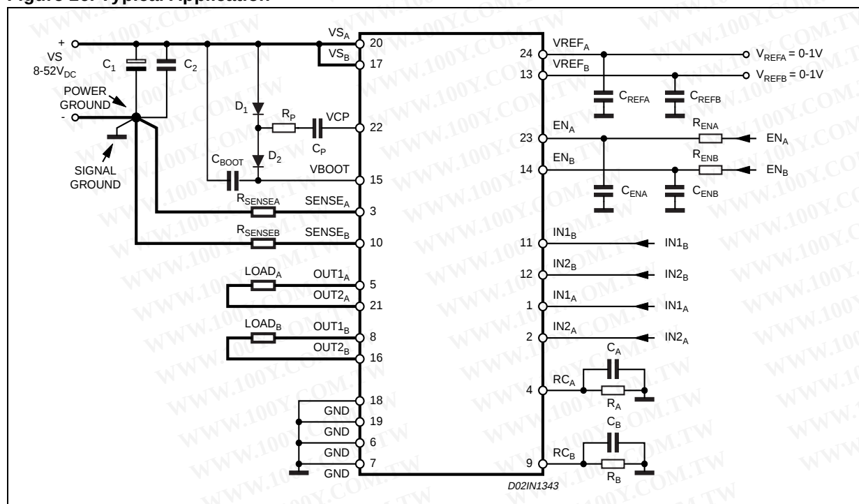
Figure 16. Typical Application
