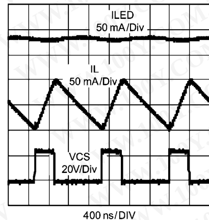
FIGURE 5. LED Ripple Current Reduction with a 1 µF Ripple Reduction Capacitor
