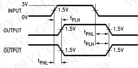
FIGURE 1. Propagation Delays
