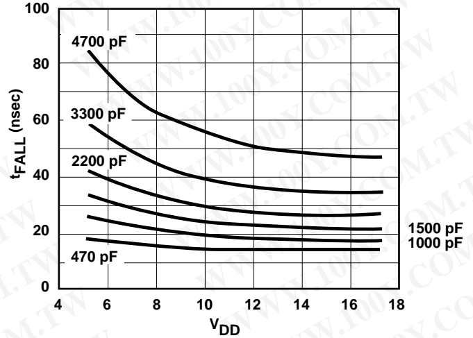
Fall Time vs. Capacitive Load
