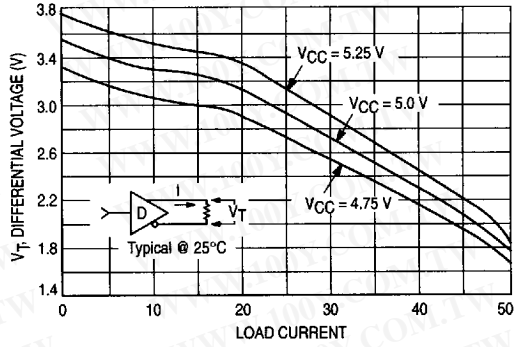
Figure 5. Driver Differential Output Characteristics
