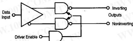
Driver Block Diagram
