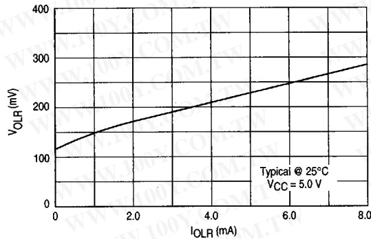
Figure 8. Receiver Output Voltage
