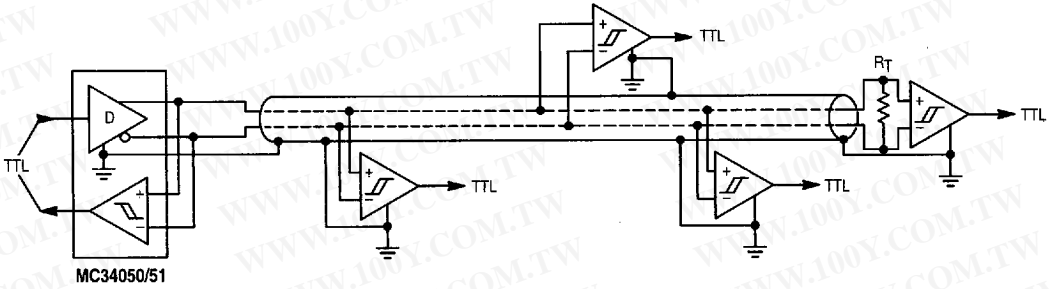
Figure 17. EIA-423 Application
