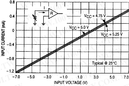
Figure 10. Receiver Input Characteristics
