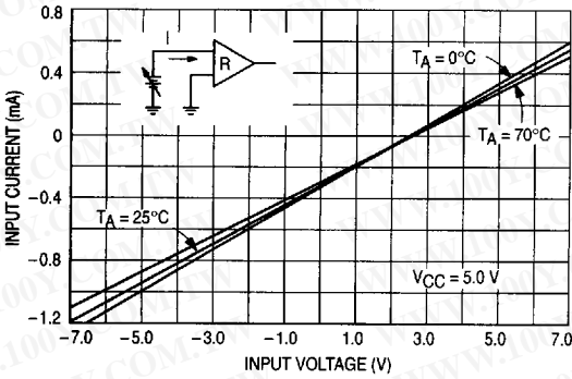
Figure 12. Receiver Input Characteristics
