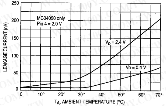
Figure 13. Receiver Output Leakage
