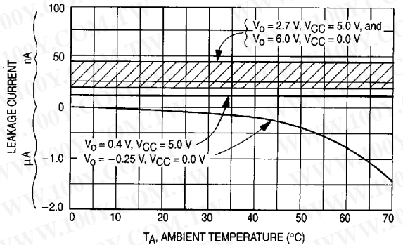
Figure 15. Driver Output Leakage
