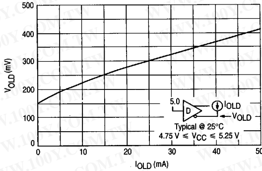
Figure 6. Driver Output Voltage
