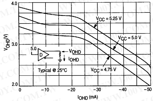
Figure 7. Driver Output Voltage
