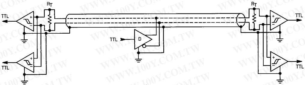
Figure 17. EIA-423 Application
