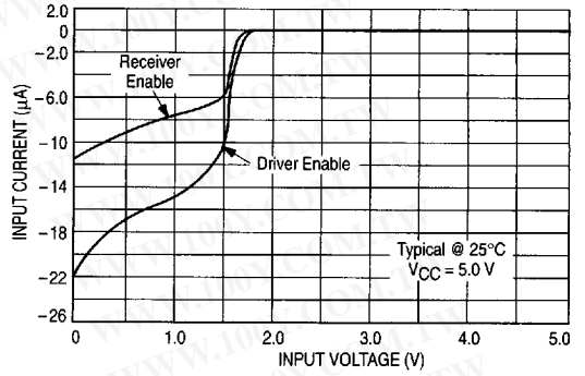
Figure 11. Enable Input Characteristics
