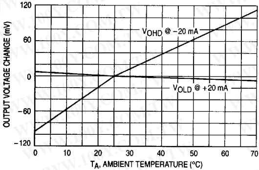
Figure 14. Driver Output Voltage
