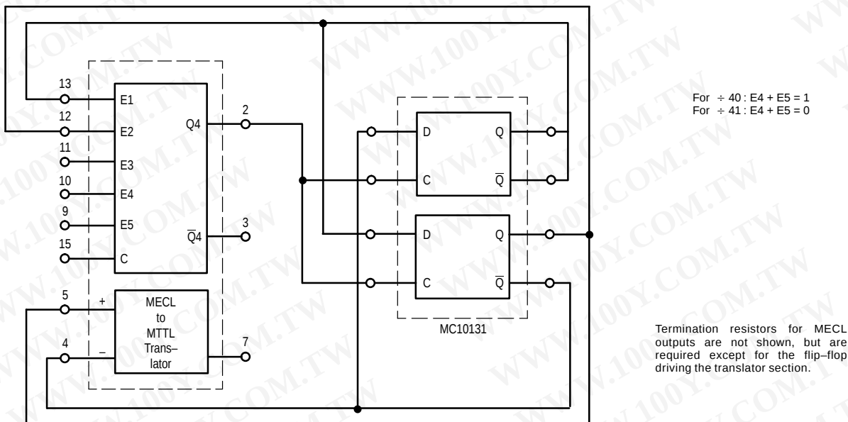
Figure 10. Divide By 40/41 (MC12013)
