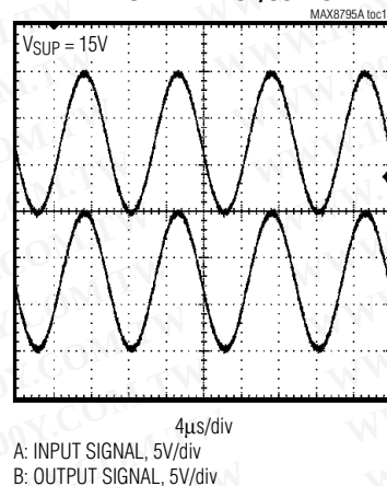
OPERATIONAL-AMPLIFIER RAIL-TO-RAIL INPUT/OUTPUT
