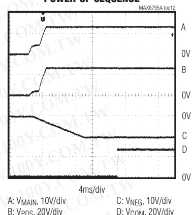
POWER-UP SEQUENCE
