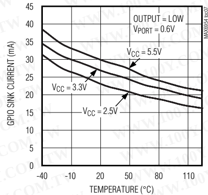
GPIO SINK CURRENT vs. TEMPERATURE
