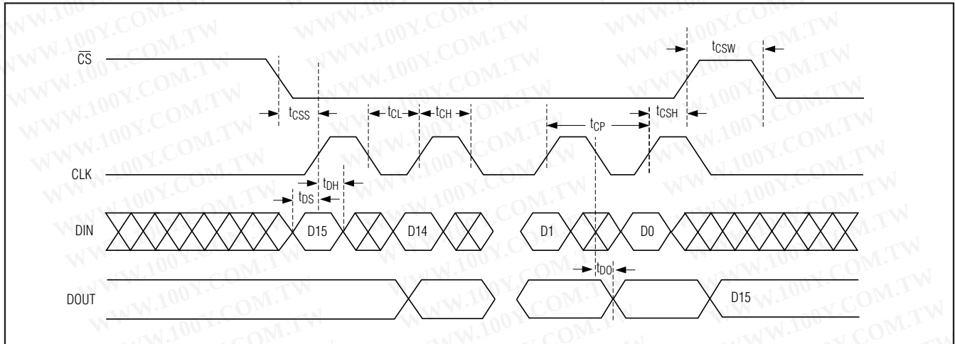
Figure 3. Timing Diagram
