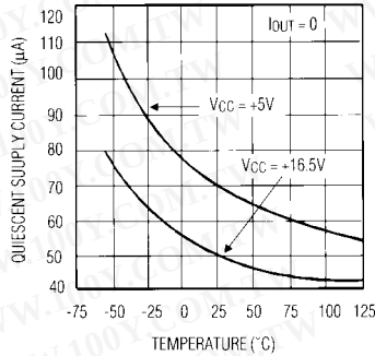
MAX620/621 QUIESCENT SUPPLY CURRENT vs. TEMPERATURE
