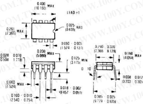
8 Lead CERDIP
