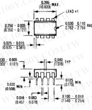
8 Lead Plastic DIP
