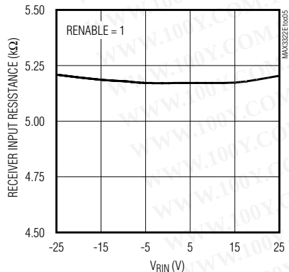
RECEIVER INPUT RESISTANCE vs. INPUT VOLTAGE RANGE
