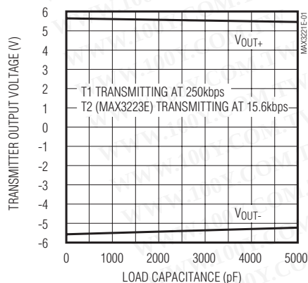
MAX3221E/MAX3223E TRANSMITTER OUTPUT VOLTAGE vs. LOAD CAPACITANCE
