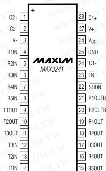
SO/SSOP/TSSOP
