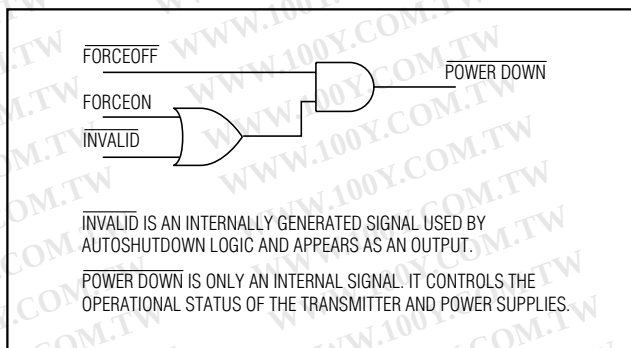
Figure 2c. AutoShutdown Logic
