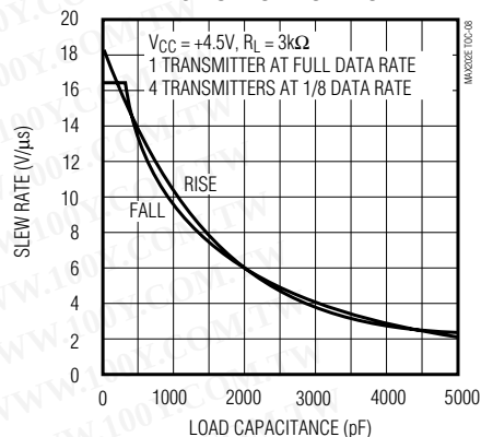
MAX205E-MAX208E TRANSMITTER SLEW RATE vs. LOAD CAPACITANCE
