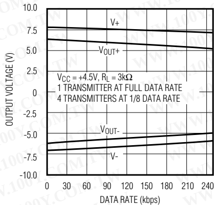
MAX205E-MAX208E OUTPUT VOLTAGE vs. DATA RATE
