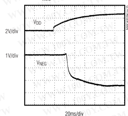
VNEG STARTUP SCOPE SHOT
