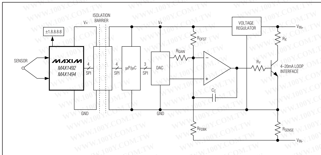
Figure 22. 4-20mA Transmitter
