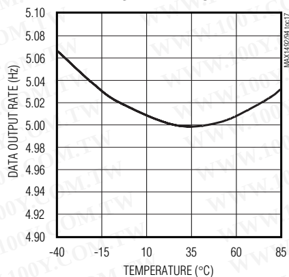
DATA OUTPUT RATE vs. TEMPERATURE
