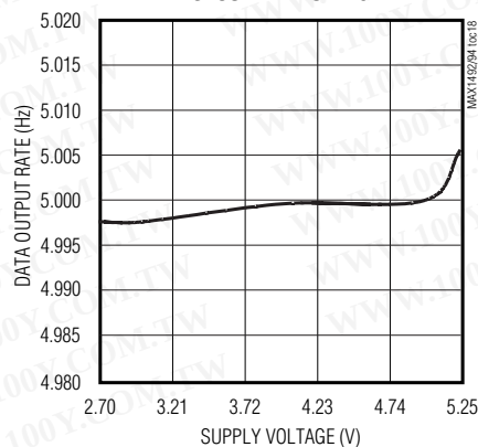
DATA OUTPUT RATE vs. SUPPLY VOLTAGE
