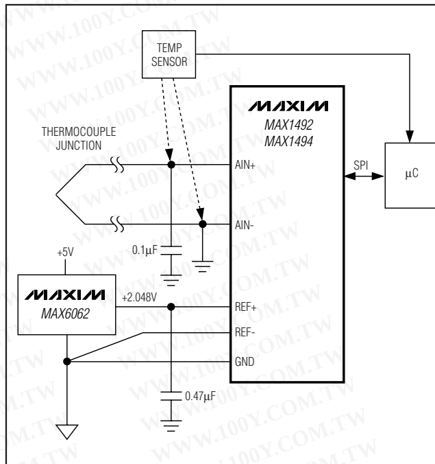
Figure 21. Thermocouple Application with MAX1492/MAX1494
