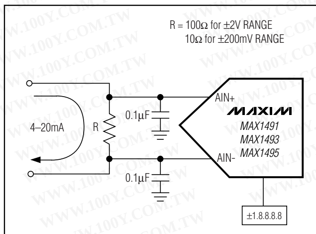
Figure 14. 4–20mA Measurement
