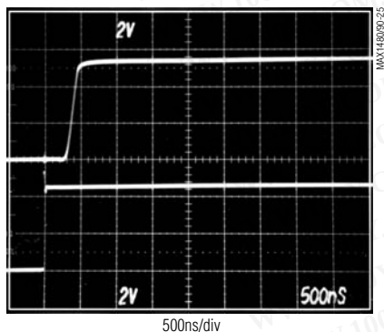
MAX1480C DRIVER ENABLE TIME
