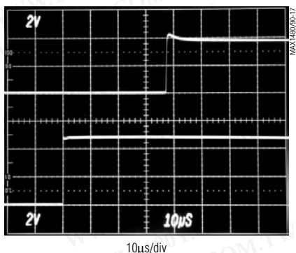
MAX1480B DRIVER ENABLE TIME
