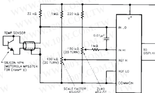
Figure 20. Digital Thermometer
