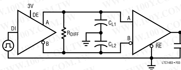
Figure 3. Driver/Receiver Timing Test Circuit
