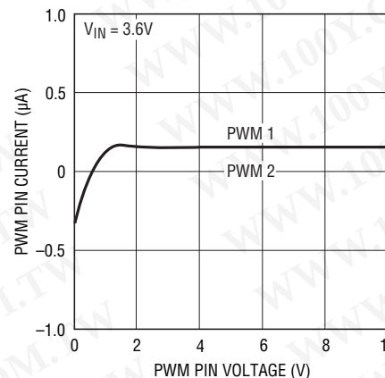
PWM Pin Input Bias Current
