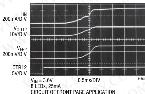
Figure 4. Start-Up Waveforms
