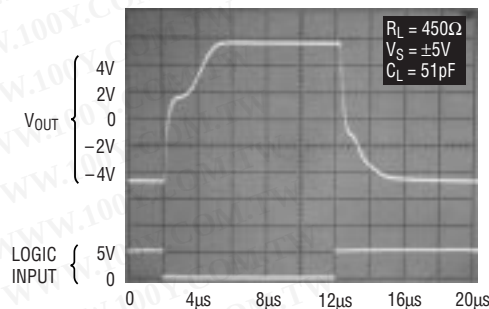
Output Waveform
