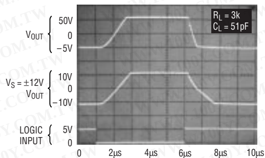
Output Waveform
