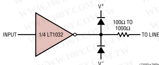
Protecting Against More Than \pm 30\text{V} Output Overload
