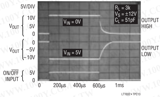
ON/OFF Response Time
