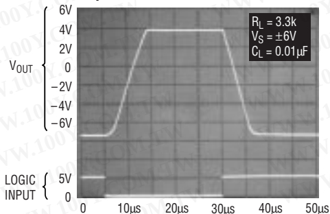
Output Waveform Driving Capacitive Load
