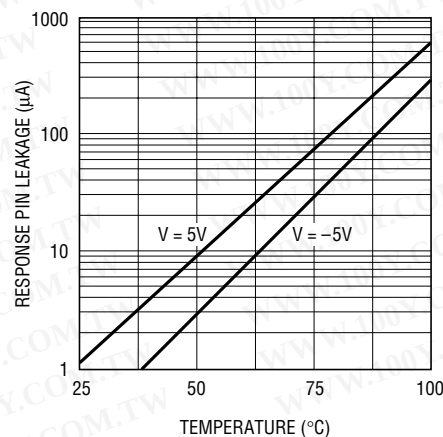
Response Pin Leakage vs Temperature (Device Off)
