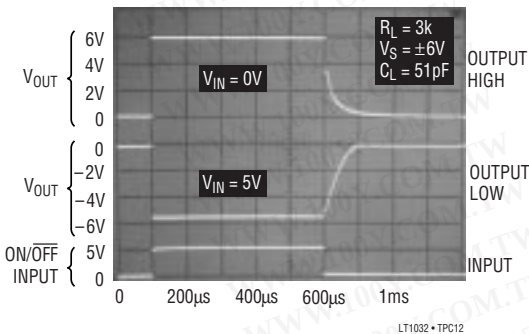
ON/OFF Response Time
