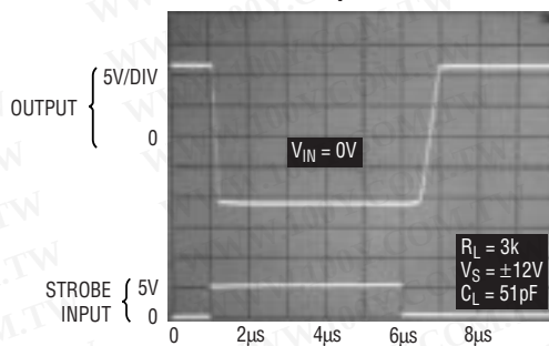
Strobe Pin Response
