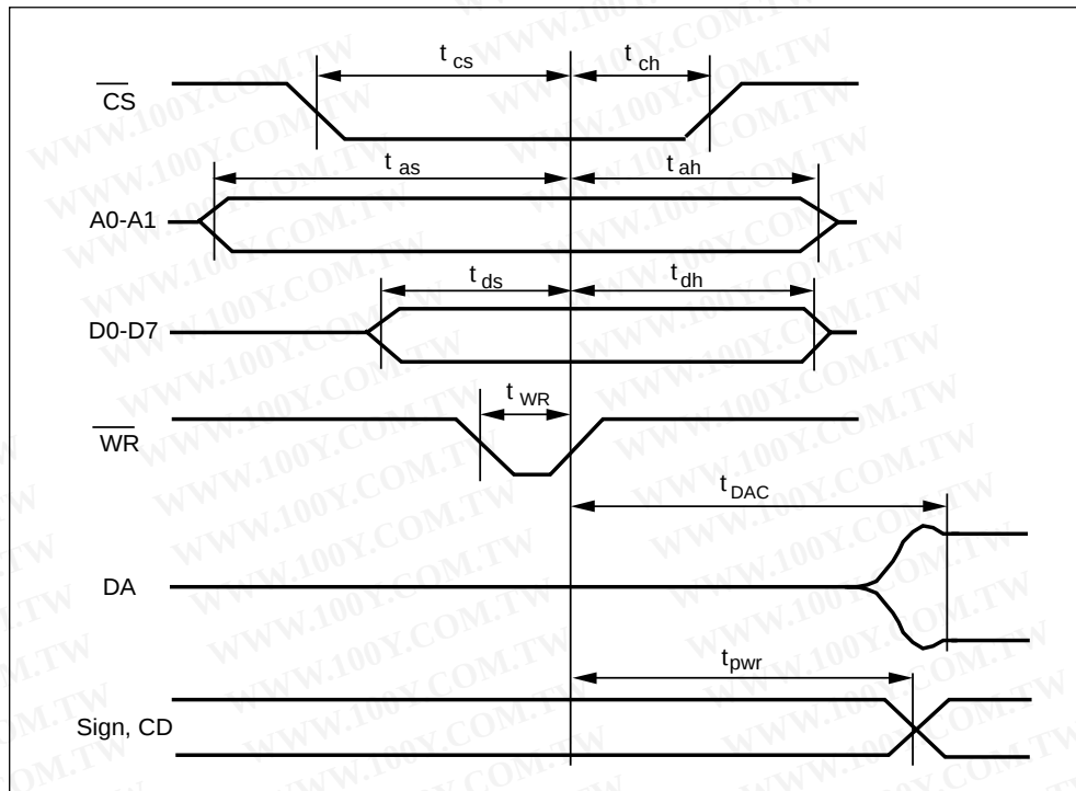
Figure 11. Timing
