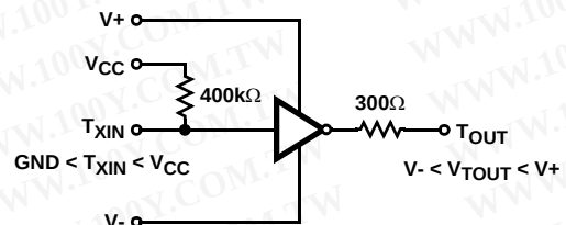
FIGURE 4. TRANSMITTER
