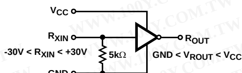
FIGURE 5. RECEIVER
