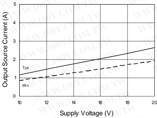
Figure 32B. Output Source Current vs. Supply Voltage
