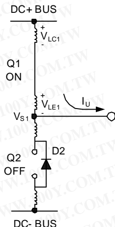
Figure 10: V_s positive
