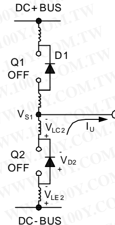
Figure 11: V_s negative
