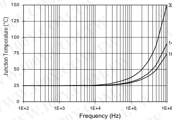
Figure 32. IRS2112S T J vs. Frequency (IRFBC20) R GATE = 33 W, V CC = 15 V
