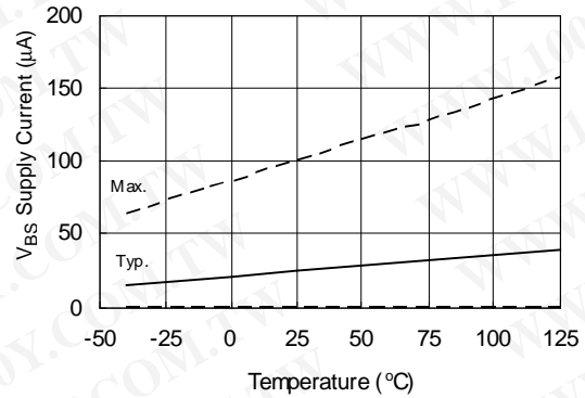
Figure 16A. V BS Supply Current vs. Temperature
